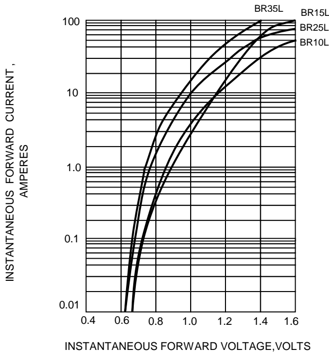
FIG.3-TYPICAL FORWARD CHARACTERISTICS
